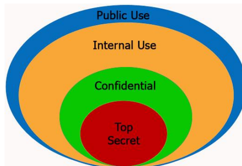
Figure 5: Data Classification
